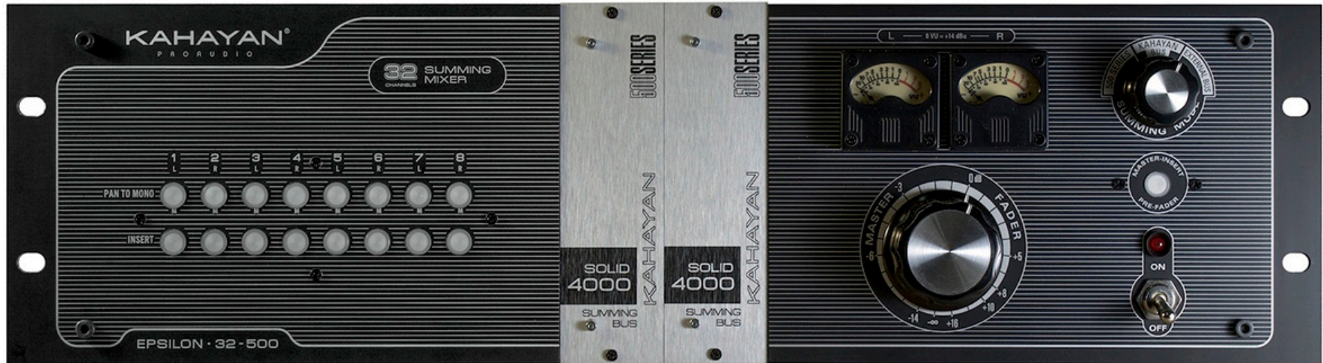
EPSILON 32-500 - FRONT PANEL
